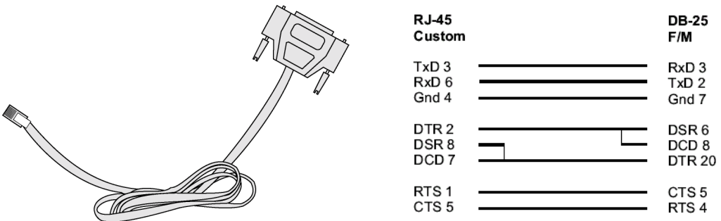
Figure 36: Cable 2 - Cyclades RJ-45 to DB-25 Female/Male, crossover
