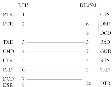
Figure 42: RJ-45 Female to DB-25 Male Adapter
