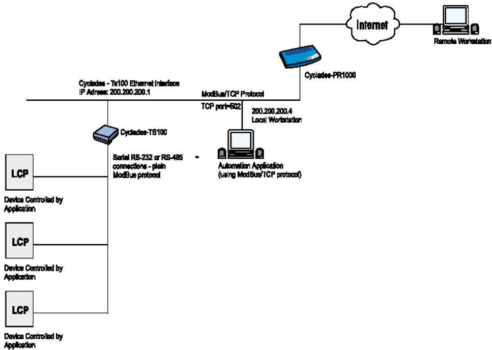
Figure 30: Modbus application
