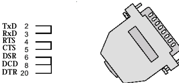
Figure 40: Loop-Back Connector
