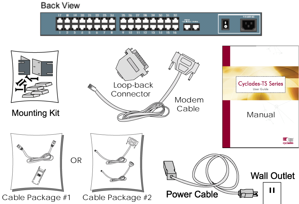
Figure 6: The Cyclades-TS2000 and cables
