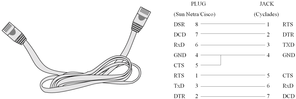
Figure 39: Cable 5 - Cyclades/Sun Netra Cable
