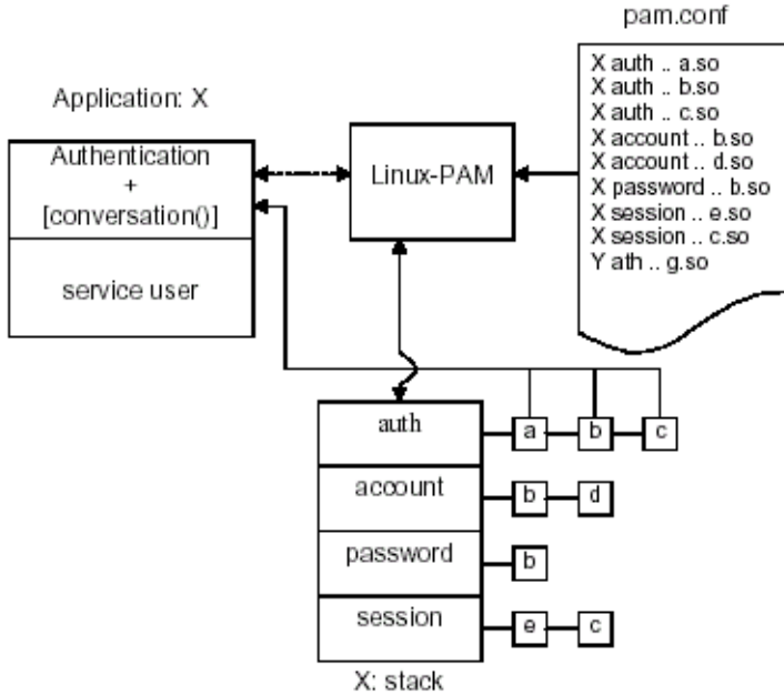
Figure 49: Data flow diagram of Linux-PAM
