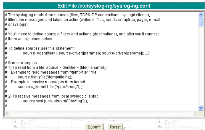
Figure 34: Syslog page 1
