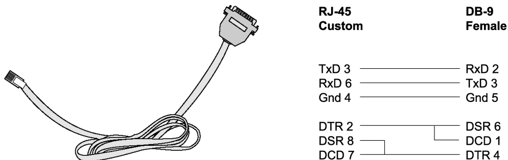
Figure 37: Cable 3 - Cyclades RJ-45 to DB-9 Female, crossover
