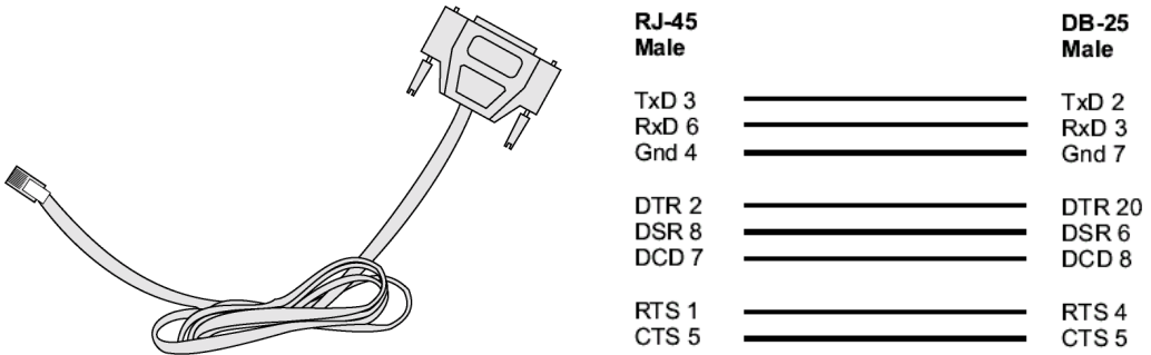
Figure 35: Cable 1 - Cyclades RJ-45 to DB-25 Male, straight-through
