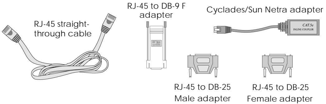
Figure 3: Cable Package #1
