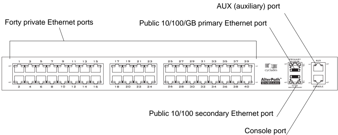
Figure 1-3: OnBoard Back With Ethernet, AUX, and Console Ports
