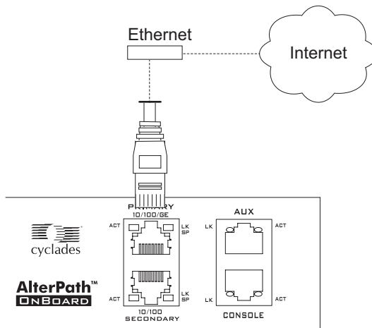
Figure 2-4: Making an Ethernet Connection to a Public Ethernet Port
