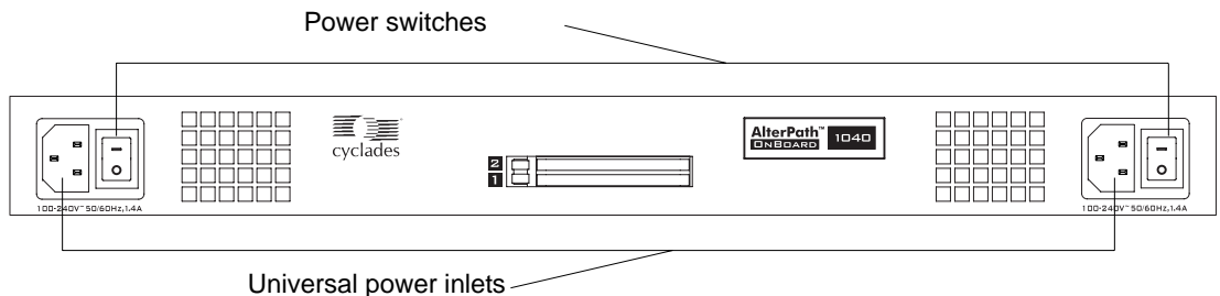
Figure 2-5: Universal AC Power Inlets and Power Switches
