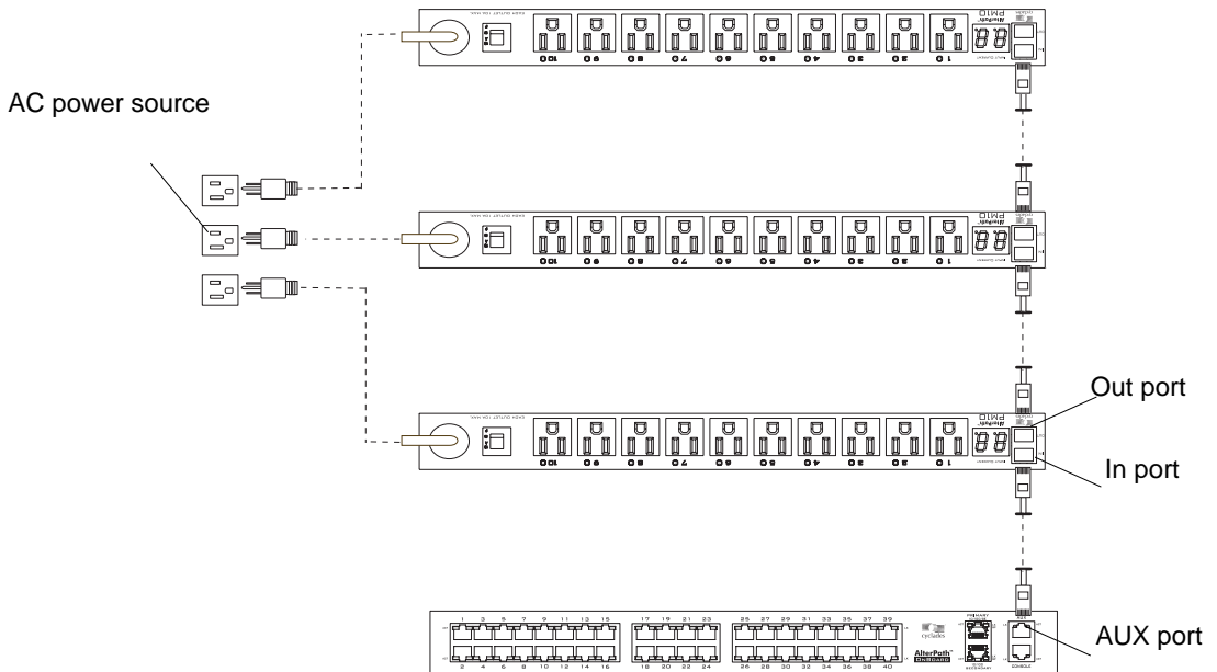
Figure 3-2: IPDUs Daisy-Chained to the AUX Port
