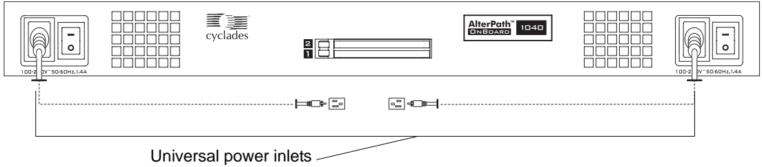
Figure 2-6: Dual AC Model Connected to Two Different Power Sources
