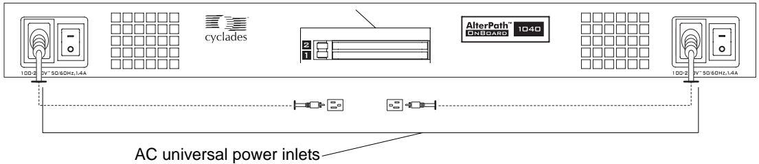
Figure 1-1: OnBoard Front With PCMCIA Card Slots and Two AC Power Inlets
