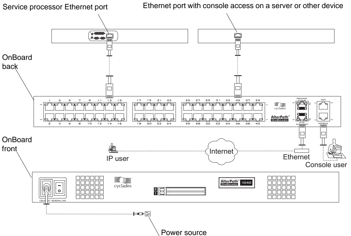
Figure 2-1: Basic Installation Connections Illustrated
