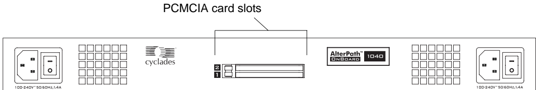
Figure 1-7: PCMCIA Slots on the OnBoard Front
