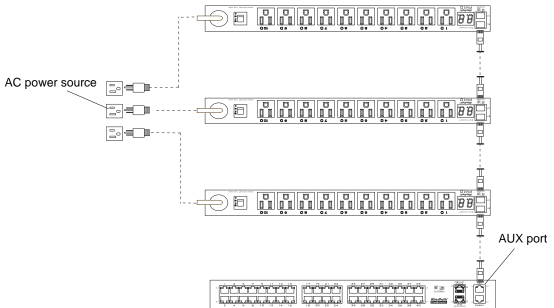
Figure 1-10: IPDUs Daisy-Chained to the AUX Port
