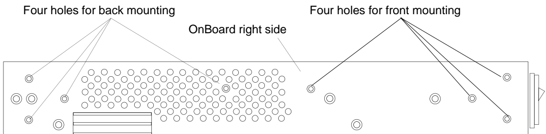
Figure 2-2: Bracket Mounting Holes on the OnBoard’s Right Side
