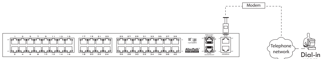
Figure 3-1: Connecting an External Modem to the AUX Port and to the Telephone Network
