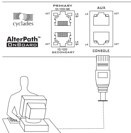
Figure 1-11: User With a Terminal Connected to the Console Port
