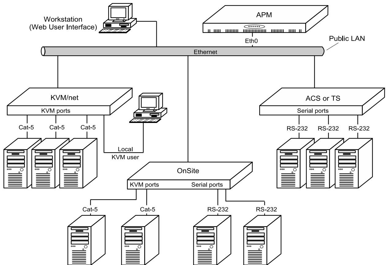
Figure 7: Single Network Setup
