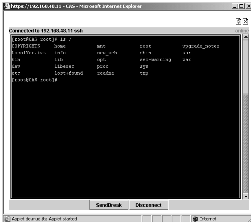
Figure 3-4: Java Applet
