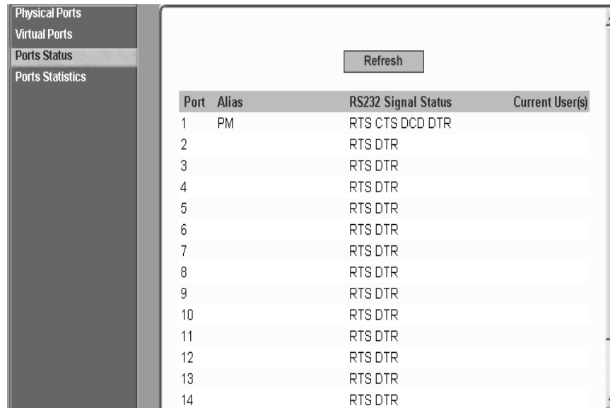
Figure 10-1: Expert > Ports
