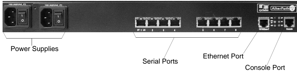
Figure 1-4: ACS Connectors
