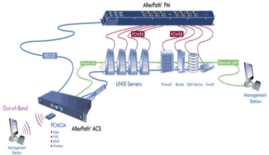
Figure 1-5: IPDU Integration With ACS
