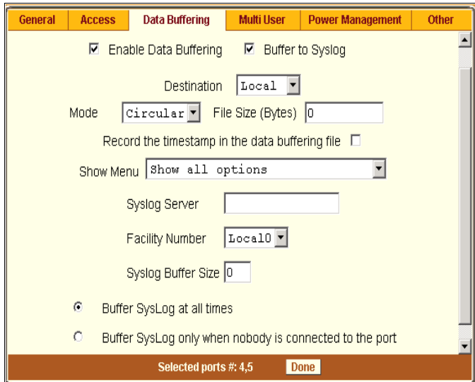
Figure 10-24: Expert > Ports > Physical Ports > Data Buffering
