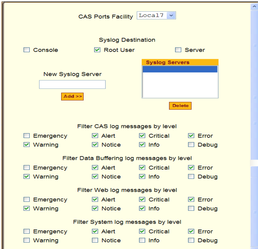
Figure 8-3: Expert > Network > Syslog
