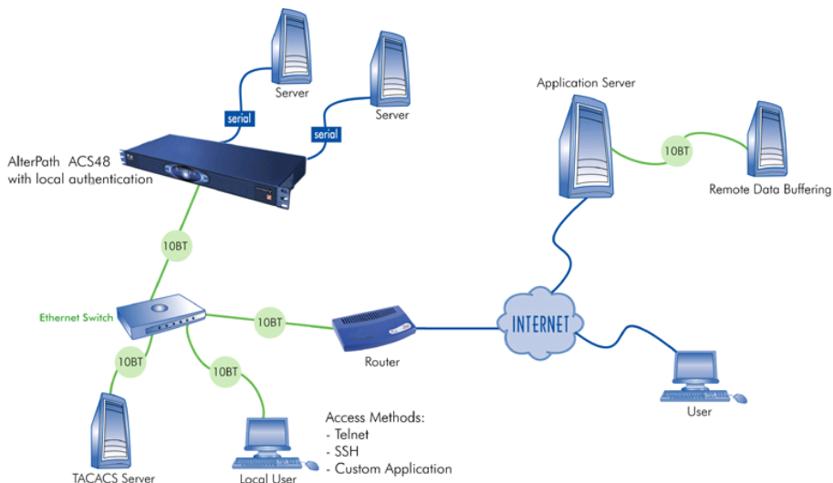
Figure 2-1: ACS Setup Example
