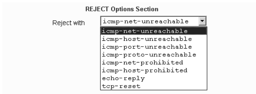
Figure 8-38: Firewall Configuration “Add Rule” and “Edit Rule” REJECT Target Menu Options
