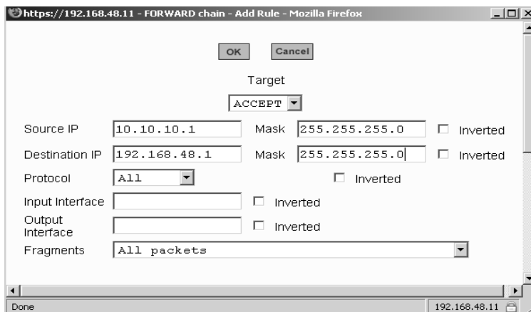
Figure 8-28: Expert > Firewall Configuration “Add Rule” and “Edit Rule” Dialog Boxes
