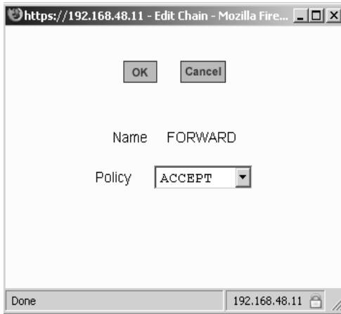
Figure 8-22: Expert > Firewall Configuration “Edit Chain” Dialog Box
