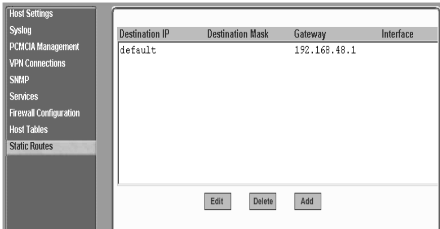
Figure 8-40: Expert > Network > Static Routes
