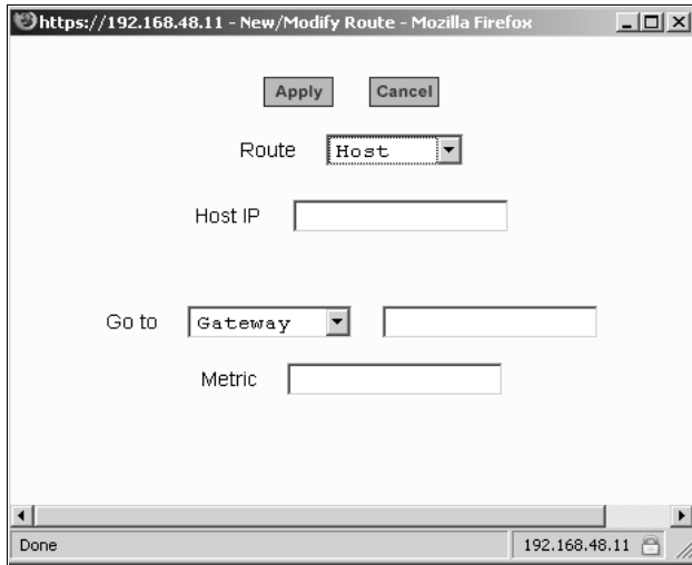
Figure 8-43: Expert > Static Routes “Add” and “Edit” Dialog Boxes - Host Route
