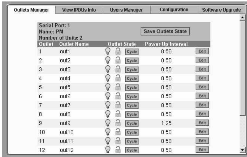
Figure 7-6: Expert > Applications > IPDU Power Mgmt. > Outlets Manager
