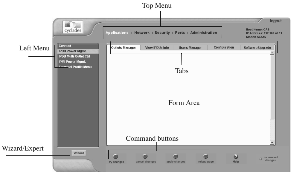
Figure 6-1: Expert Mode Screen Elements
