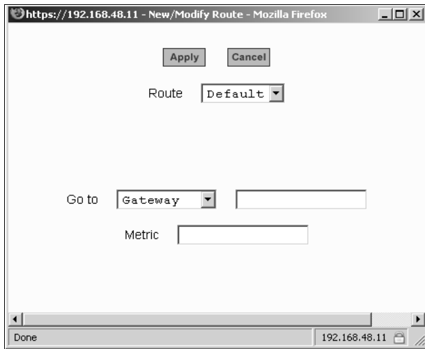
Figure 8-41: Expert > Static Routes “Add” and “Edit” Dialog Boxes - Default Route
