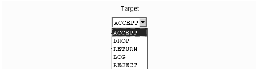
Figure 8-29: Firewall Configuration “Add Rule” and “Edit Rule” Target Menu Options
