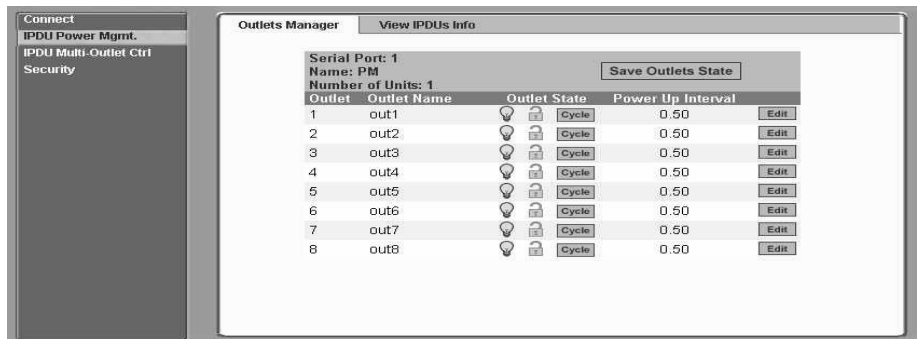
Figure 3-5: Regular User > IPDU Power Mgmt. Forms
