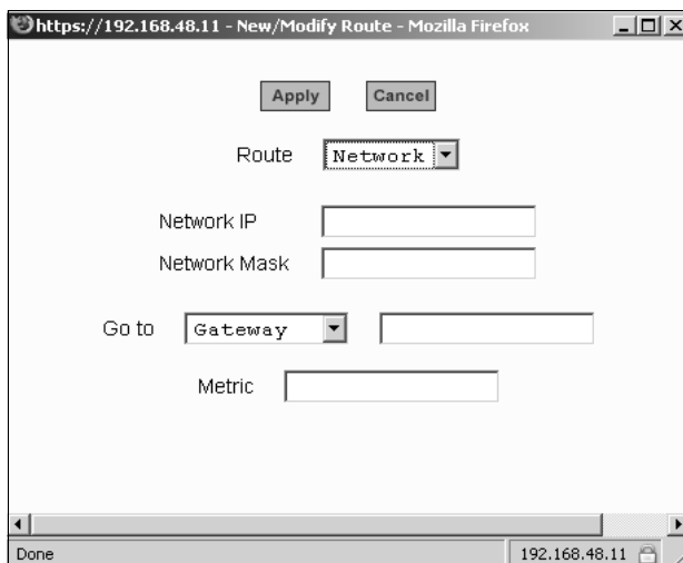
Figure 8-42: Expert > Static Routes “Add” and “Edit” Dialog Boxes - Network Route
