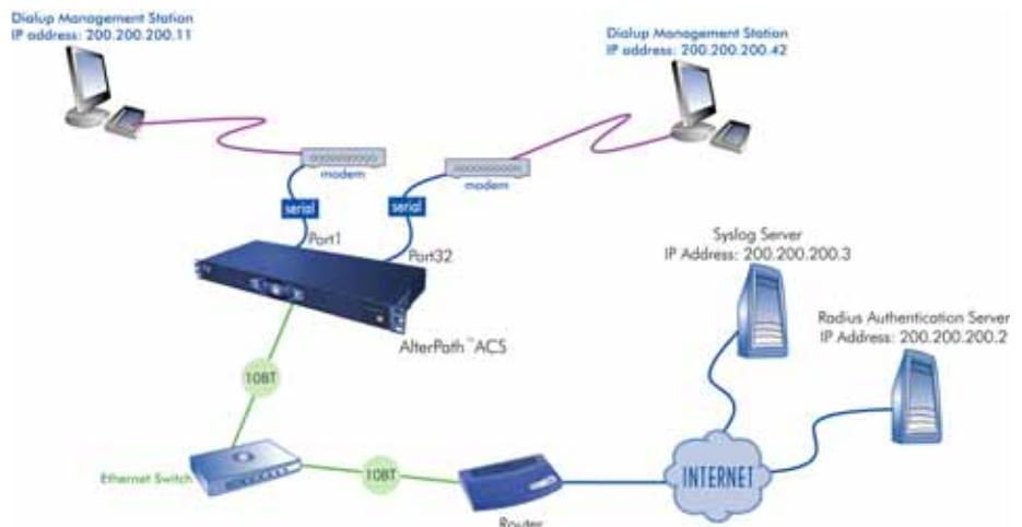
Figure 7.4 - Ports configured for dial-in access
