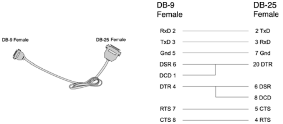
Figure C.19 - Cable 3 for the ACS1 - DB-9 Female to DB-25 Female, crossover
